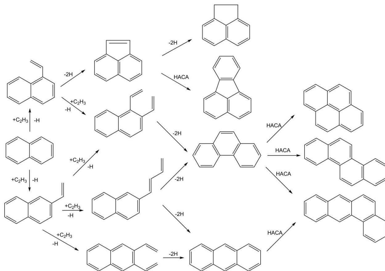
Fig. 6. HACA reactions from naphthalene.
