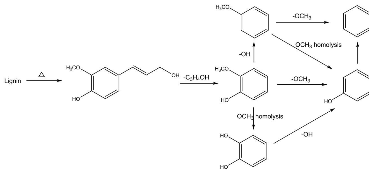
Fig. 4. Mechanisms of coniferyl alcohol degradation.
