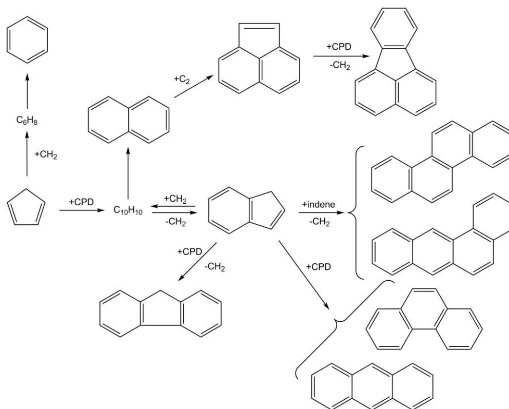
Fig. 8. Formation of PAH from CPD and indene.
